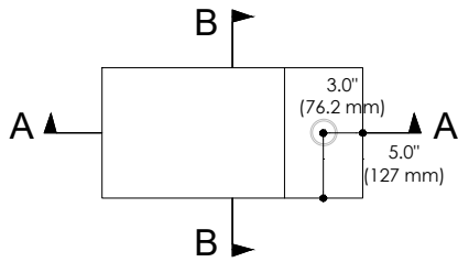
PLAN VIEW
