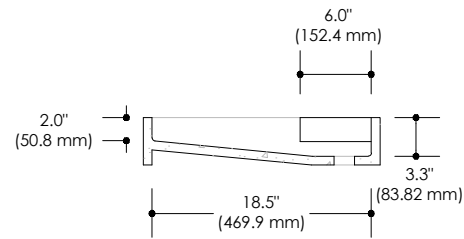
SECTION A
