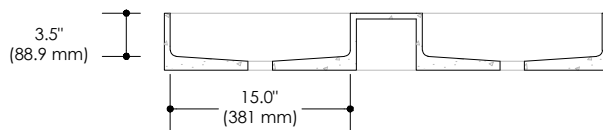
SECTION A
