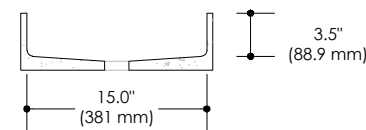
SECTION B
