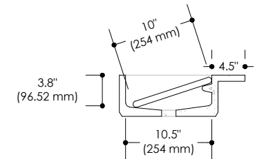
SECTION A
