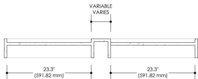
SECTION A
