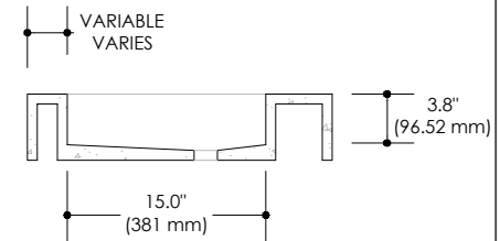
SECTION B
