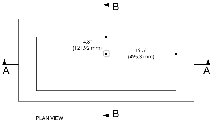
PLAN VIEW
