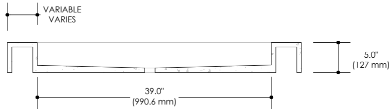
SECTION A
